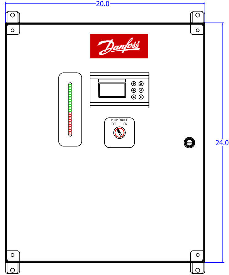
FRONT VIEW OF ENCLOSURE ENCLOSURE 24"(H) X 20"(W) X 8"(D)
